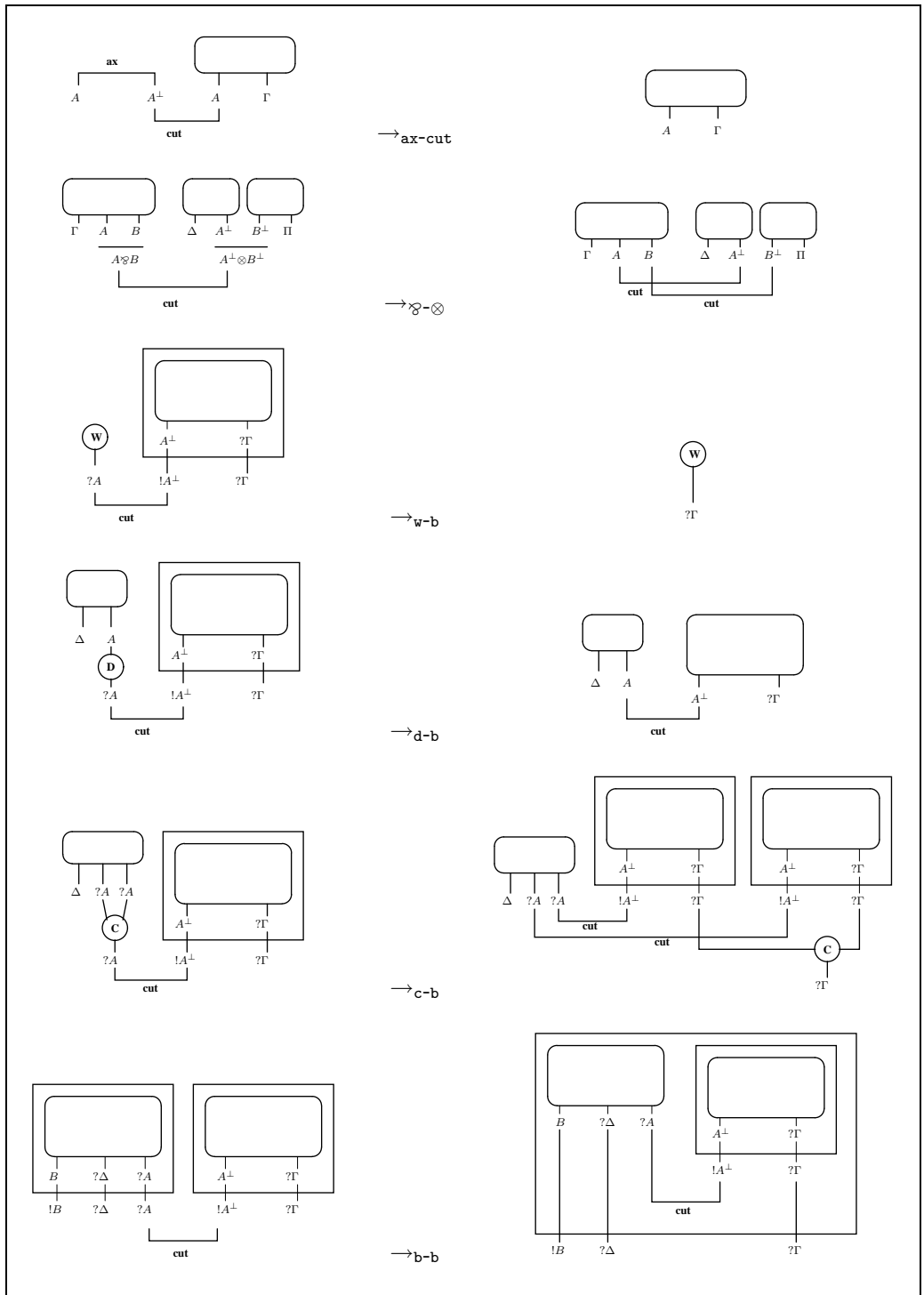
Figure 1: Cut elimination rules for MELL Proof-nets
