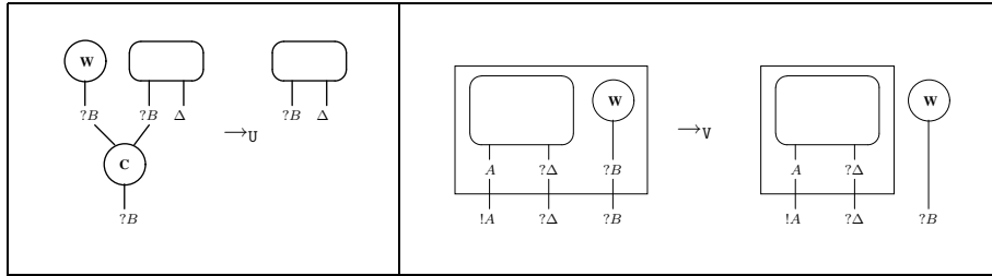
Figure 2: Extra reduction rules for MELL proof-nets
