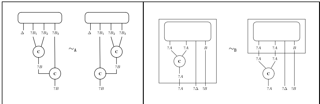
Figure 3: Equations for MELL proof-nets
